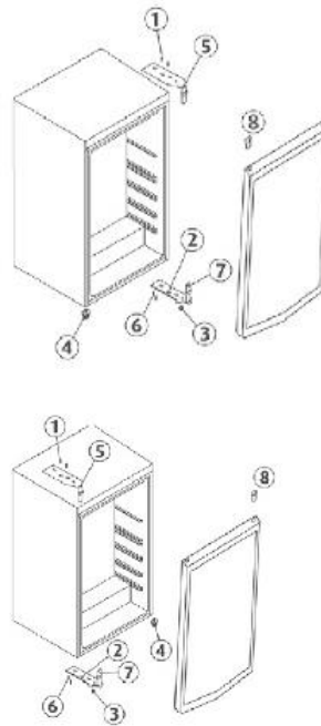
Fig 1 Position of components prior to reversal of the door hinge. Fig 2 Position of components after reversal of the door hinge.
